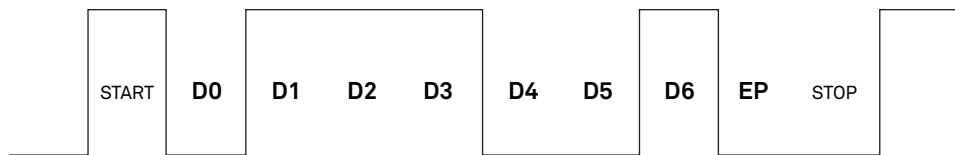
Figure 6 Example SDI-12 transmission of the character 1 (0x31)
