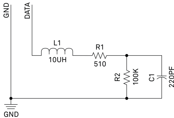
Figure 4 Equivalent circuit diagram
