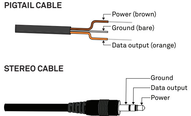
Figure 3 Connection types
