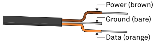
Figure 3 Pigtail wiring
