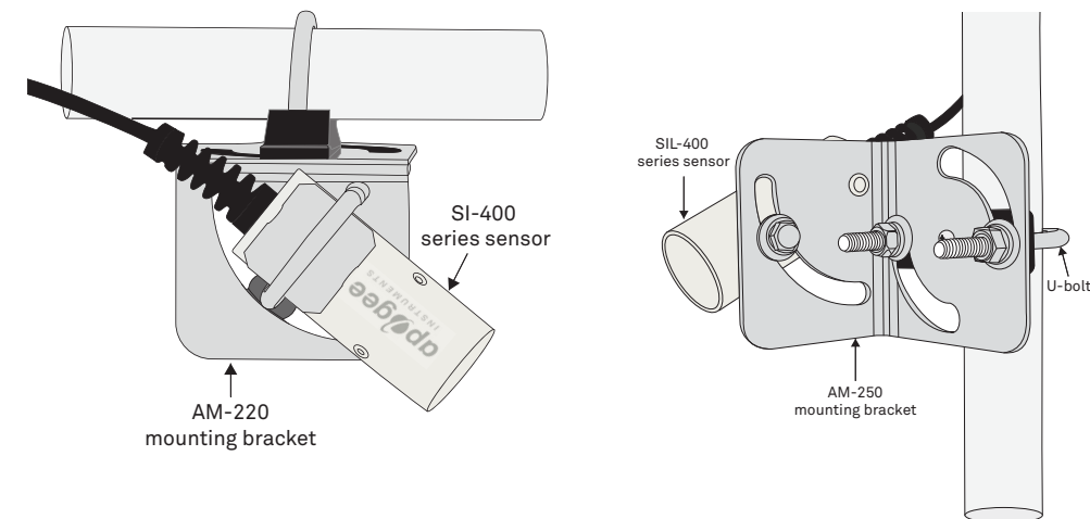
Figure 2 Apogee IR sensor and mounting bracket
