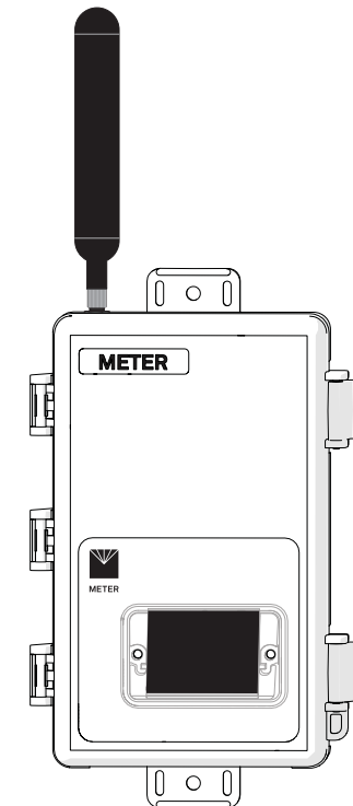
Figure 9 EM60G data logger exterior. EM60 is identical, without an antenna.
