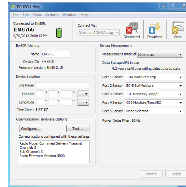
Figure 3 ECH20 Utility Main screen
