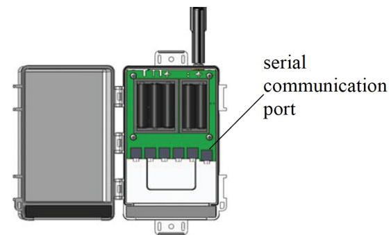
Figure 2 Port diagram
